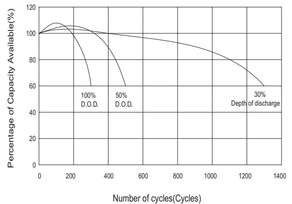
Number of cycles Vs. Depth of Discharge
