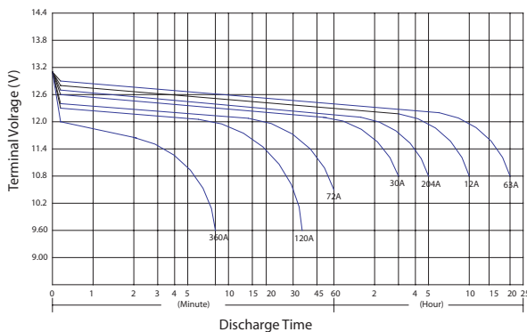
Discharge Characteristics (25°)
