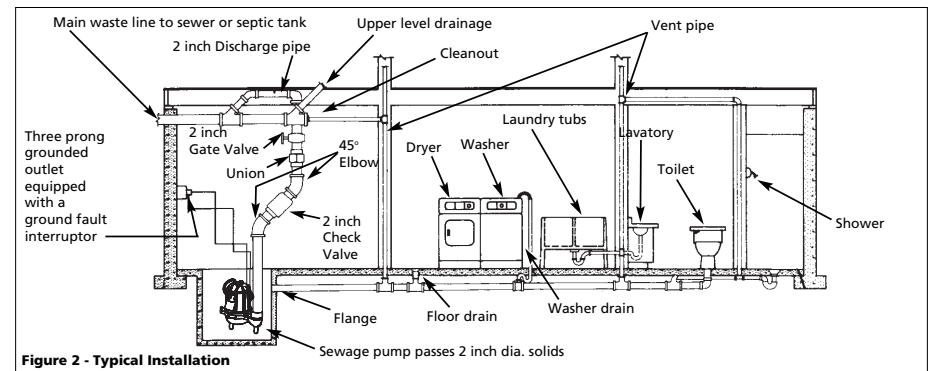
Figure 2 - Typical Installation
