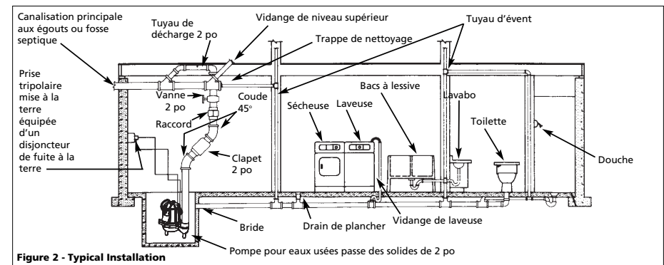
Figure 2 - Typical Installation
