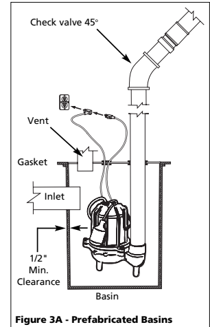
Figure 3A - Prefabricated Basins
