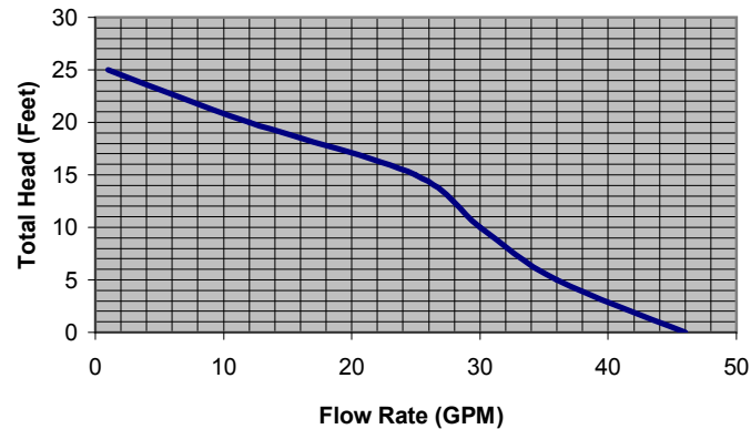
PERFORMANCE CURVE
